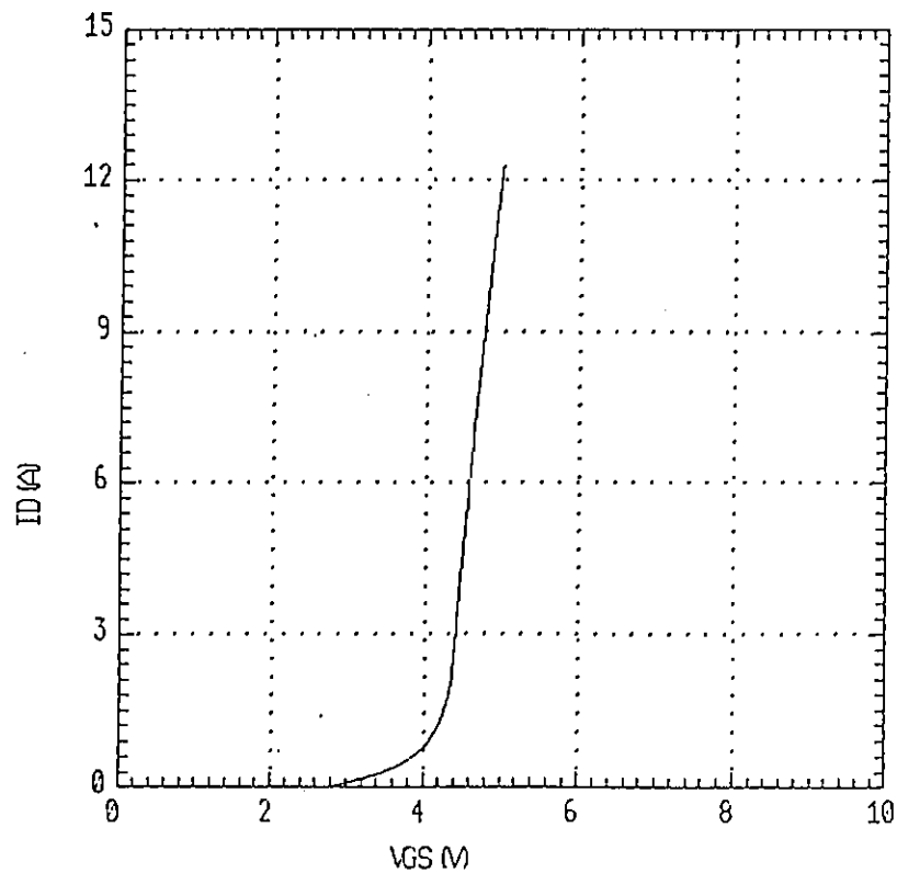
Typical Transfer Characteristics I_D = f(V_{GS}) : 80 \mu s pulse test, V_{DS} = 25V , T_{ch} = 25^\circ\text{C}
