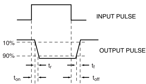
WAVE FORMS
