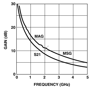
Figure 26. AT-32033 Gains vs. Frequency at V_{CE} = 5\text{ V} , I_C = 20\text{ mA} .
