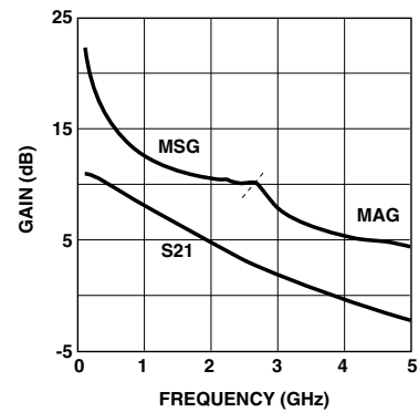
Figure 17. AT-32011 Gains vs. Frequency at V_{CE} = 1 \text{ V} , I_C = 1 \text{ mA} .
