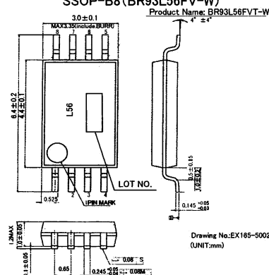
Fig4-(i) PHYSICAL DIMENSION TSSOP-B8 (BR93L56FVT-W)
