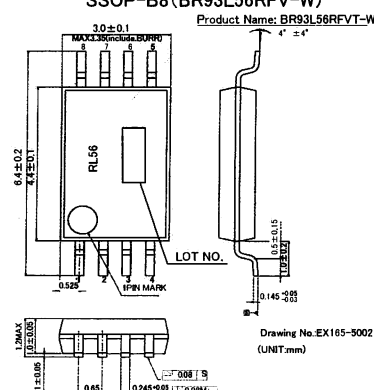
Fig4-(j) PHYSICAL DIMENSION TSSOP-B8 (BR93L56RFVT-W)
