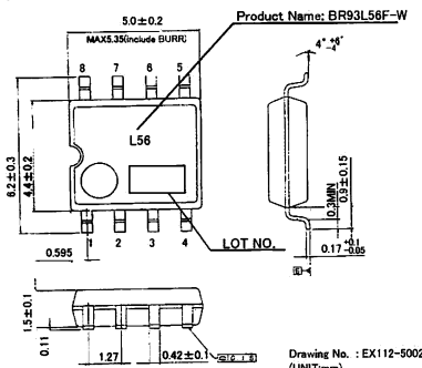
Fig4-(a) PHYSICAL DIMENSION SOP8 (BR93L56F-W)
