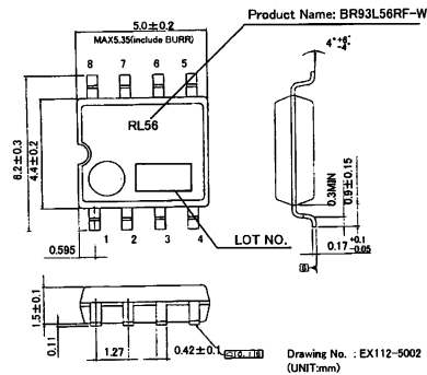
Fig4-(b) PHYSICAL DIMENSION SOP8 (BR93L56RF-W)
