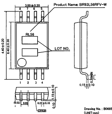
Fig4-(h) PHYSICAL DIMENSION SSOP-B8 (BR93L56RFV-W)
