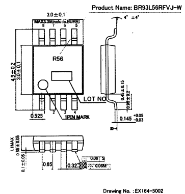
Fig4-(f) PHYSICAL DIMENSION TSSOP-B8J (BR93L56RFVJ-W)
