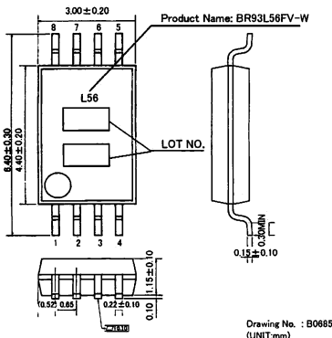
Fig4-(g) PHYSICAL DIMENSION SSOP-B8 (BR93L56FV-W)
