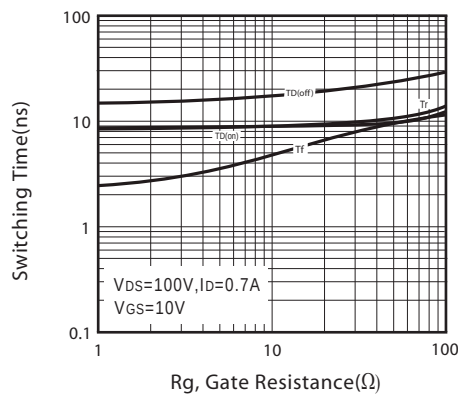
Figure 11. switching characteristics
