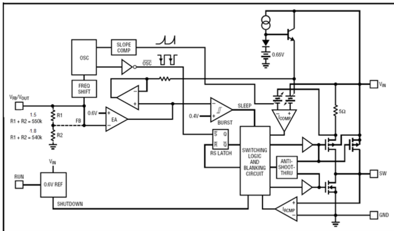
Figure2:Functional Block Diagram of TD6811
