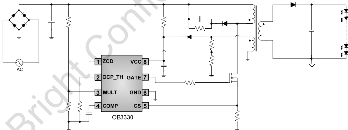
Figure1: OB3330 Typical Application Schematic
