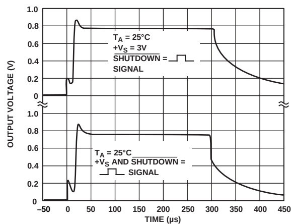
Figure 16. V_{OUT} Response Time to \overline{SHUTDOWN} Pin and +V_S Pin vs. Time
