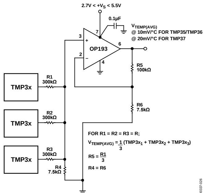
Figure 28. Configuring Multiple Sensors for Average Temperature Measurements
