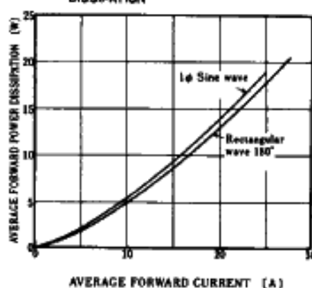
FIG.2-AVERAGE FORWARD POWER DISSIPATION
