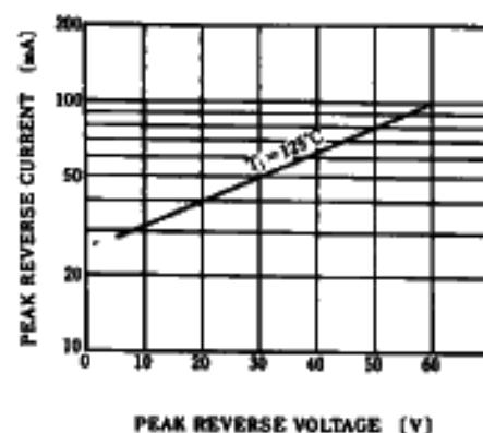
FIG.3-PEAK REVERSE CURRENT VS. PEAK REVERSE VOLTAGE
