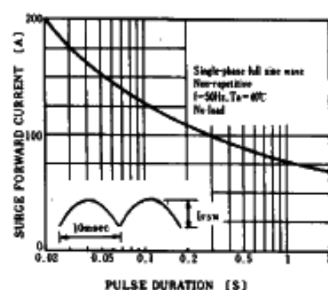
FIG.6-SURGE CURRENT RATINGS
