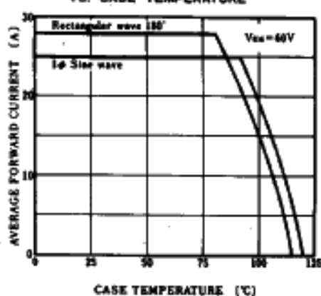
FIG.5-AVERAGE FORWARD CURRENT VS. CASE TEMPERATURE
