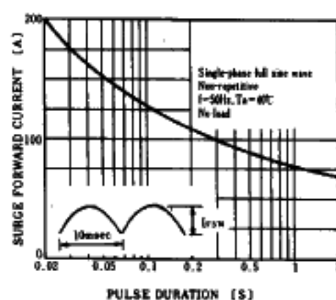
FIG.6-SURGE CURRENT RATINGS
