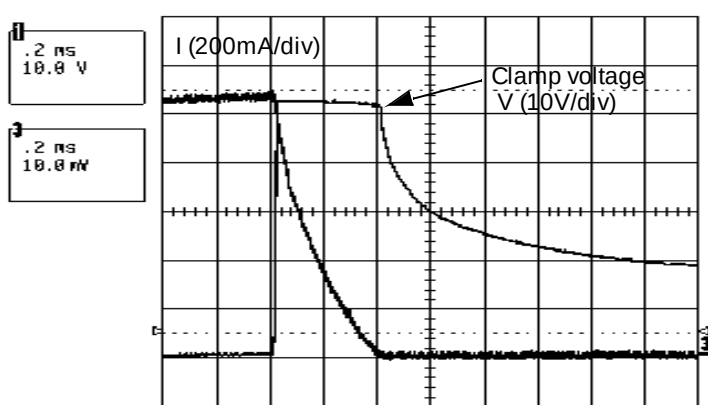
Figure17- Inductive Switching
