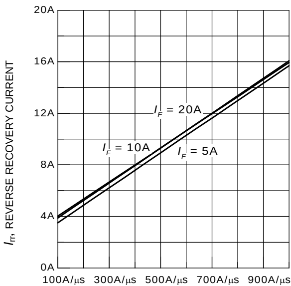
Figure 23. Typical reverse recovery current as a function of diode current slope
