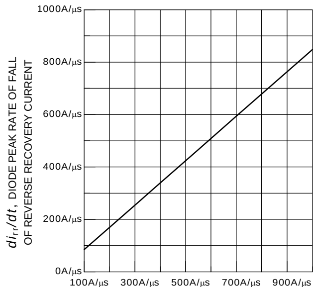
Figure 24. Typical diode peak rate of fall of reverse recovery current as a function of diode current slope
