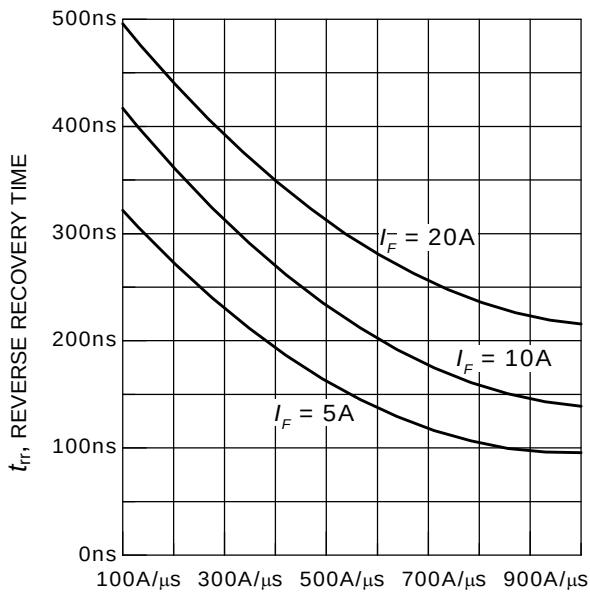
Figure 21. Typical reverse recovery time as a function of diode current slope
