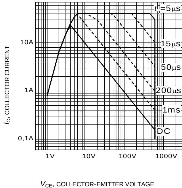
Figure 2. Safe operating area
