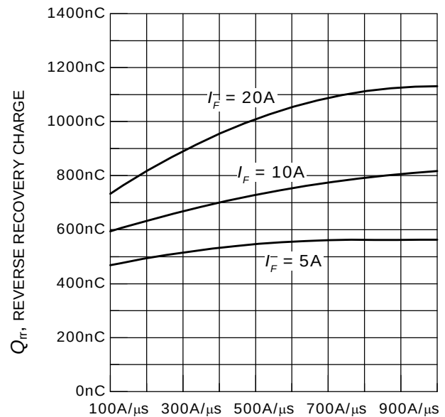
Figure 22. Typical reverse recovery charge as a function of diode current slope
