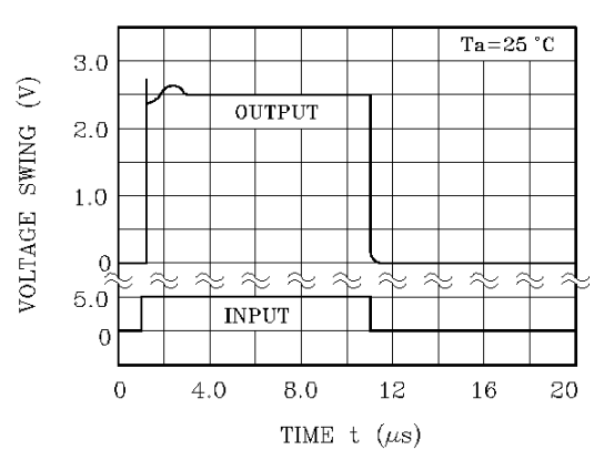
PULSE RESPONSE
